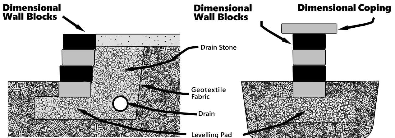
RETAINING WALL
